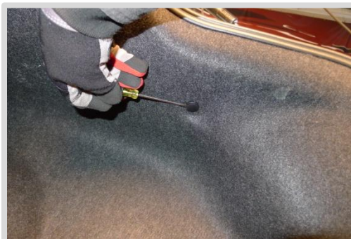
23. Remove plastic clip securing trunk liner
