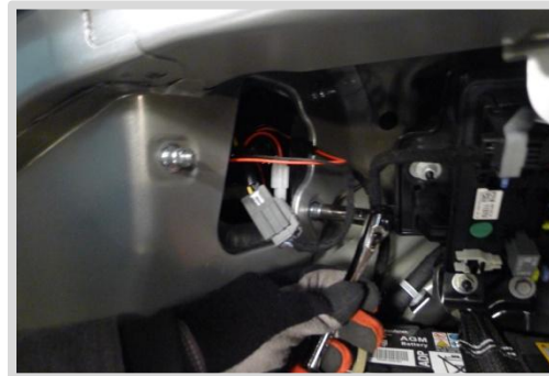
36. Remove 2 7mm bolts then the plastic handle
