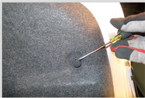
37. Remove 4 plastic clips
