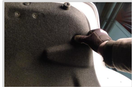
54. Replace trunk liner and 4 plastic clips
