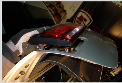
49. Remove factory taillight
