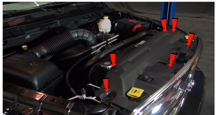
2) Remove [6x] plastic retainers securing the filler panel.
