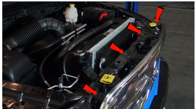
4) Remove [4x] 10mm bolts securing the grille.
